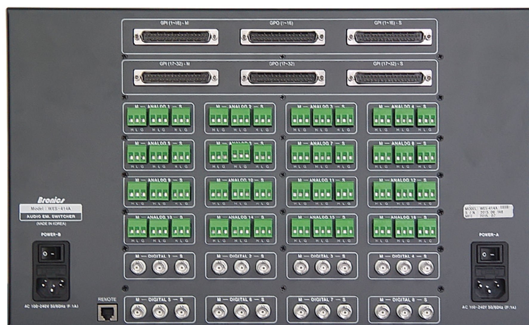
WES-414A Audio Emergency Switcher(Rear View)
