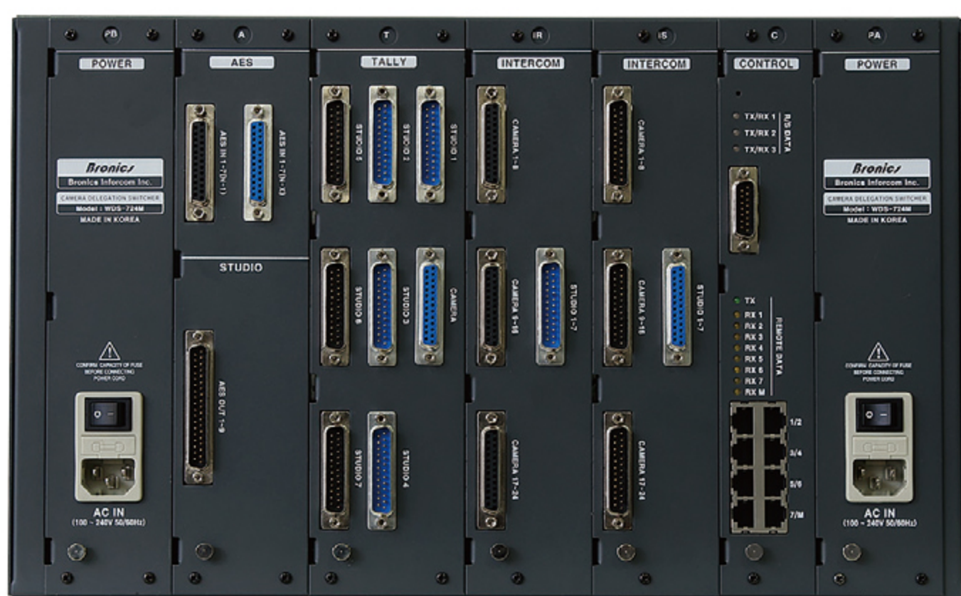
WDS-724M Rear View
