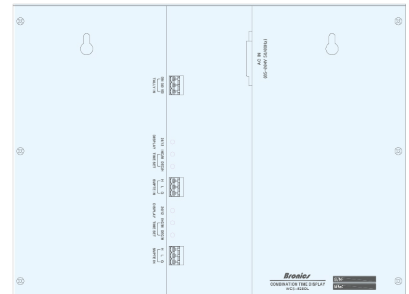
WCS-532OL Rear View
