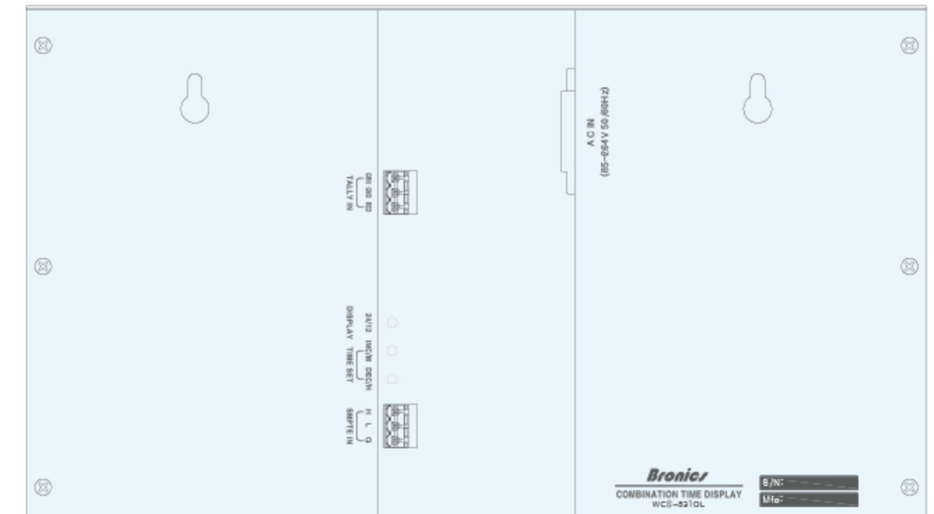
WCS-531OL Rear View
