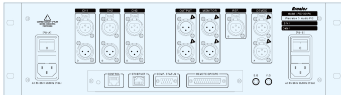
Rear View
